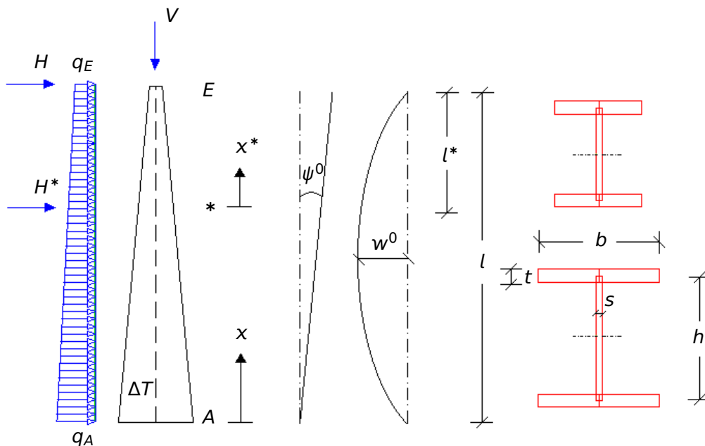
Figure 1: Problem Description
