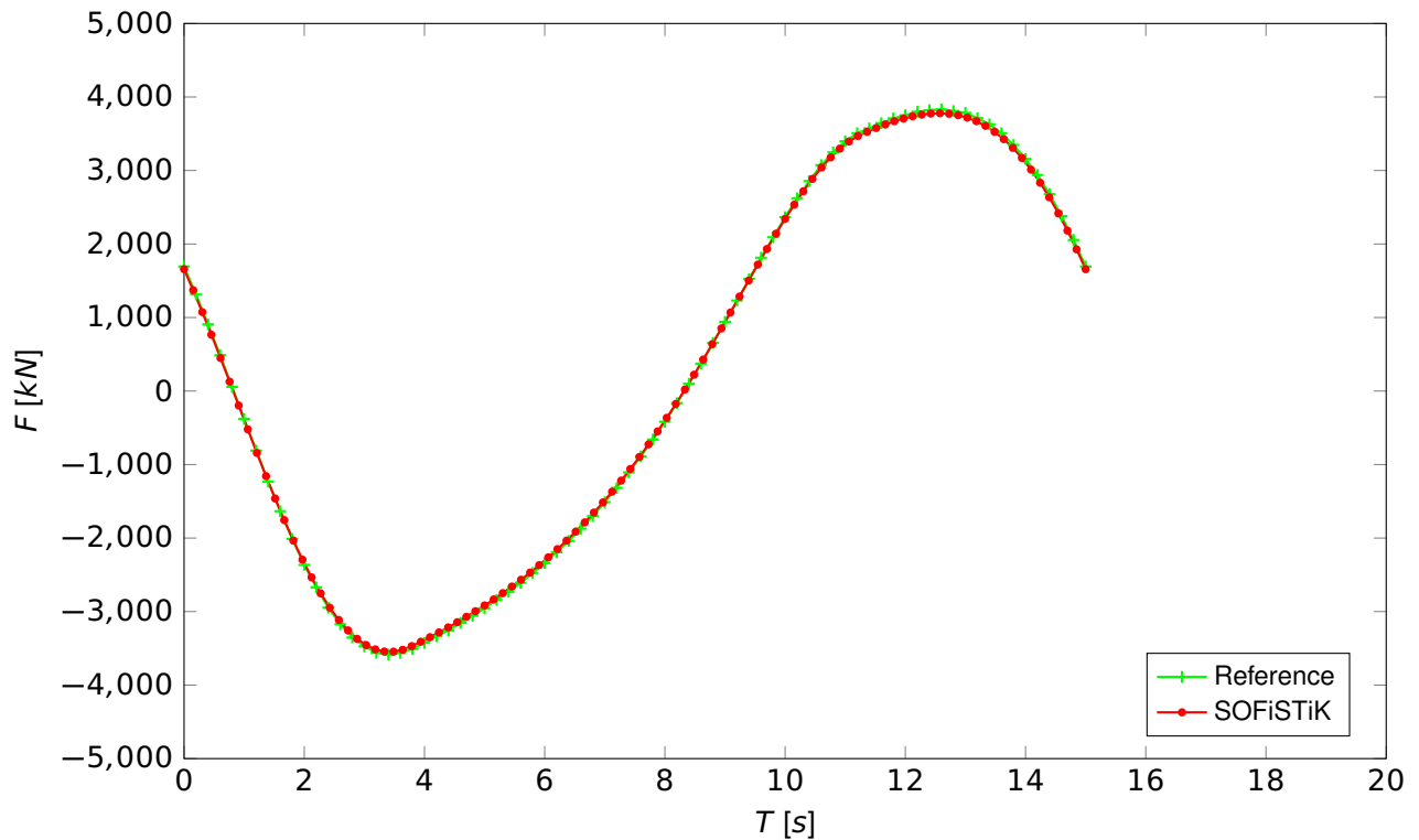
Figure 3: Accumulated Force for Airy linear wave theory in combination with Wheeler Stretching
