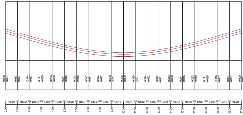
Figure 5: Tendon Geometry
