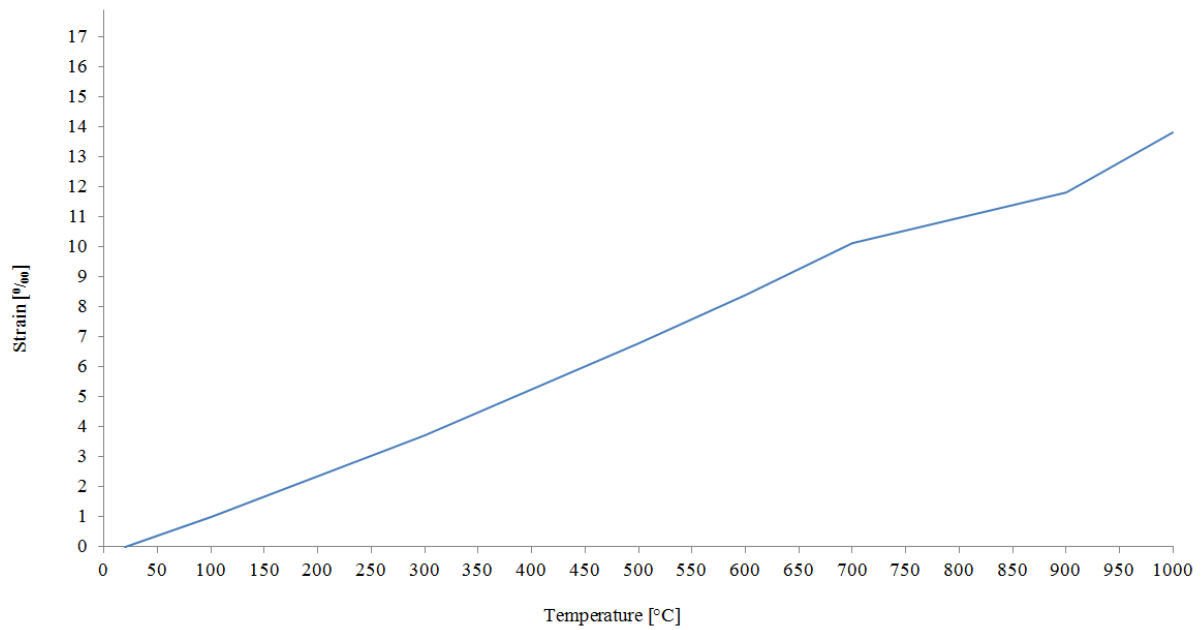
Figure 2: Temperature Strains
